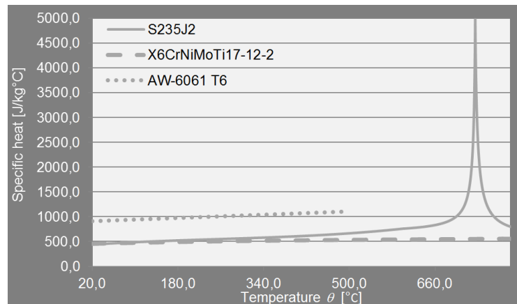
Fig. 5. Specific heat for the analysed metals
