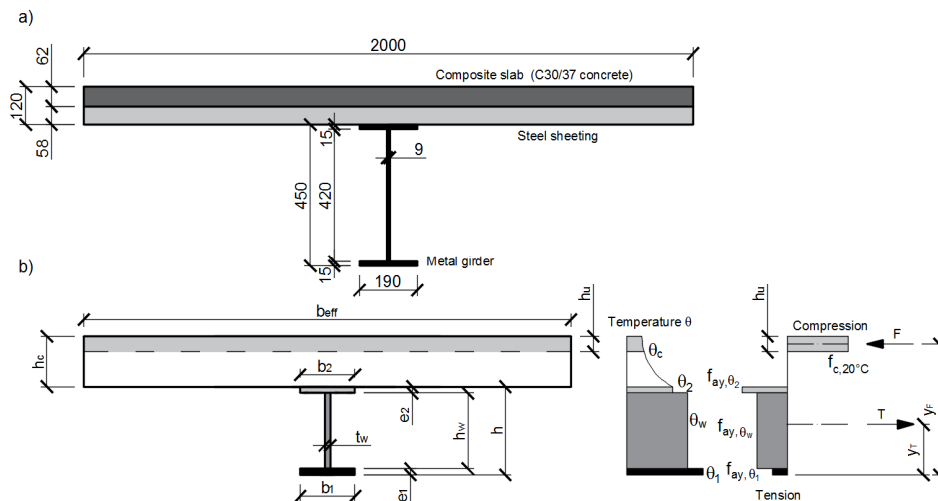
Fig. 3. a) The cross-section of the analysed composite beams, b) The model used to calculate the sagging moment resistance
