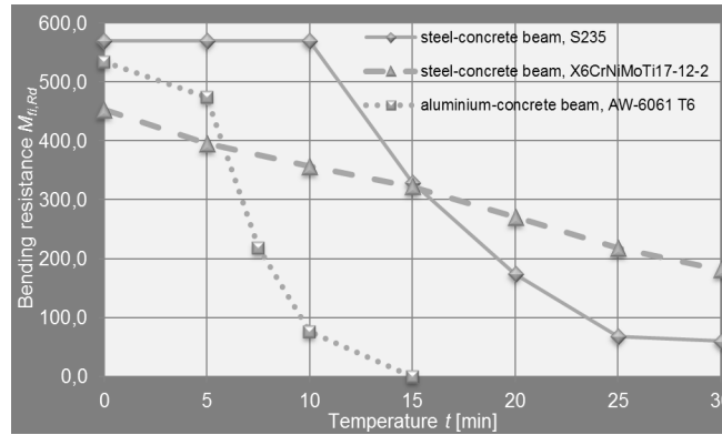
Fig. 7. Bending resistance of the composite beams in the tree-car fire
