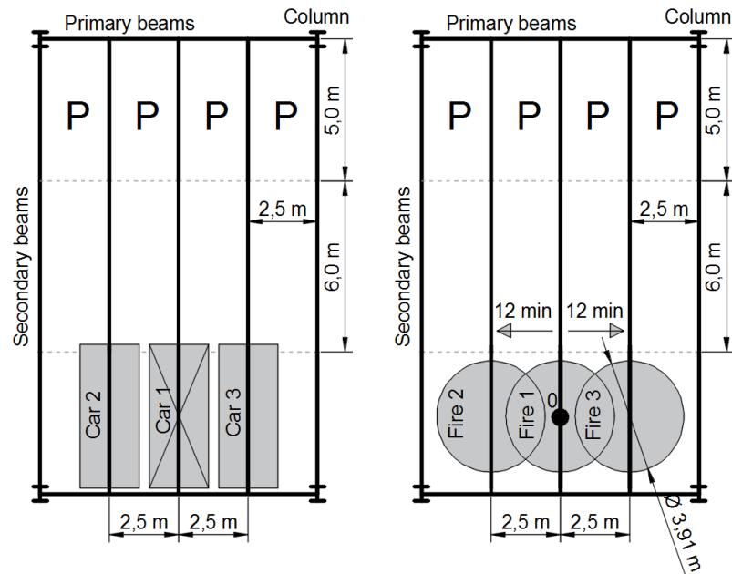
Fig. 1. Fire scenario – three cars in a line
