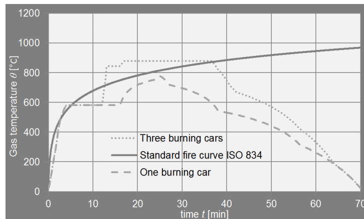
Fig. 4. Gas temperatures
