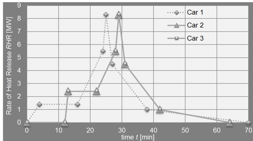
Fig. 2. Rate of heat release for each of the three cars
