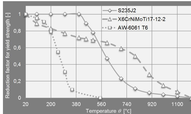
Fig. 6. Reduction factors for yield strength
